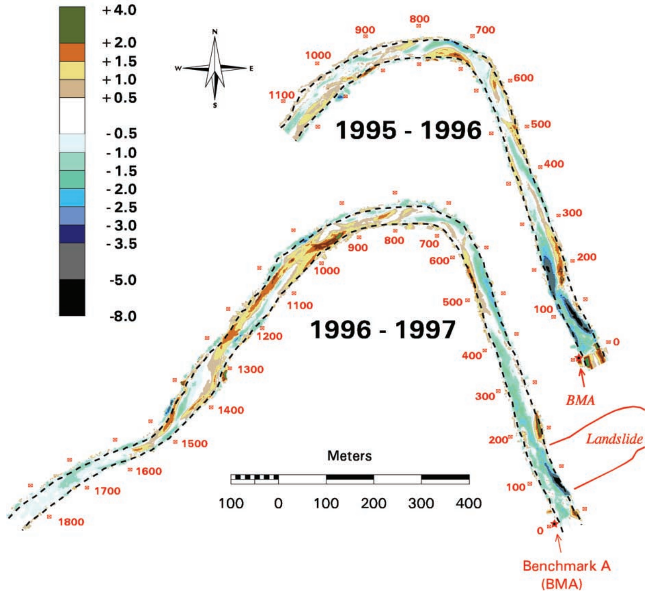
Figure 7. Depths of scour and fill in the downstream limb of the sediment wave.
