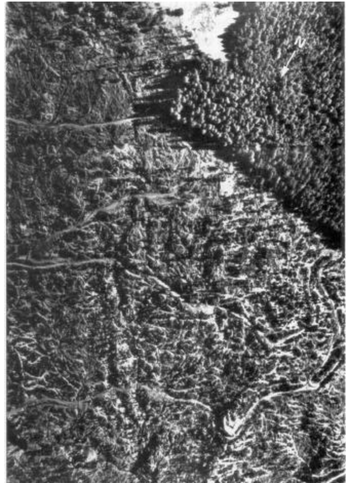
FIGURE 4.—Vertical aerial photograph taken March 7, 1972, of the western portion of the South Copper Creek study site. Note the degree of ground disturbance and the complex pattern of skid trails associated with clearcut tractor-yarding completed in 1971. Old-growth forest (upper right, outside study site) was logged the following year.
