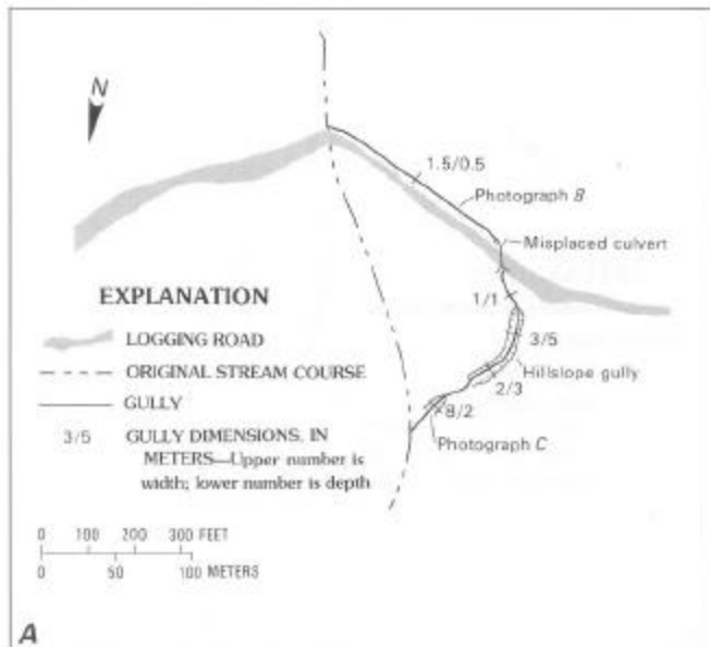
← FIGURE 8.—Gully attributed to misplaced culvert on logging road. A , Planimetric map showing diversion of a perennial watercourse down the roadside ditch for a distance of 150 m to the misplaced culvert, downslope from which a larger gully was formed. Cross-sectional dimensions of the gully are shown at selected intervals, and the computed gully volume is 1,200 m 3 . B , Photograph of a gullied roadside ditch on a logging road. C , Photograph of gully, which is much larger than gully in B above, on hillslope. Note the increase in the cross-sectional area of the gully as slope steepens.
