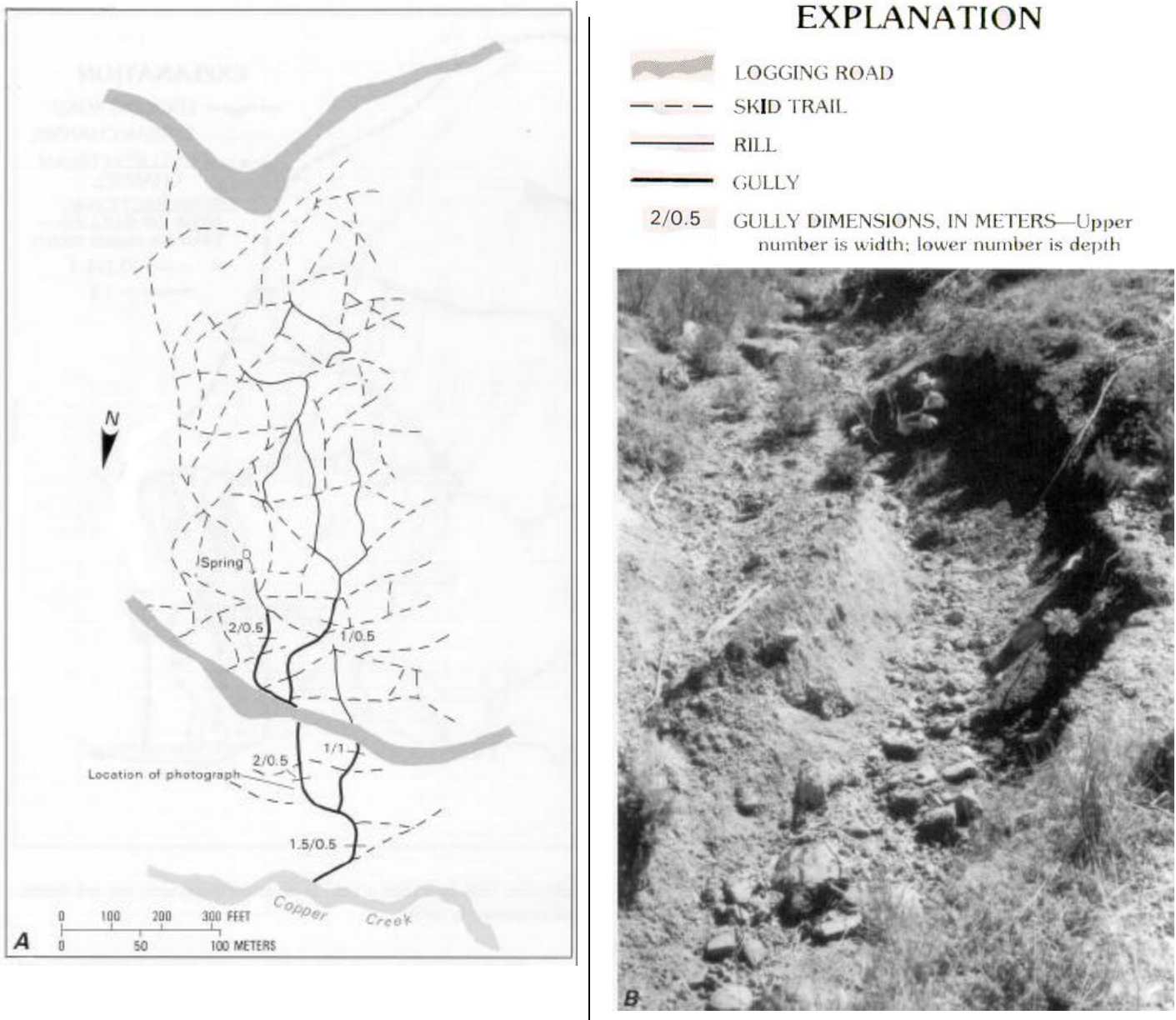
FIGURE 9.—Gullies created by increased surface runoff over the skid-trail network in a tractor-yarded area. A, Planimetric map showing gully system caused by concentrated runoff flowing on skid trails. Note the comparatively small gully dimensions shown on the map. Total gully erosion from the network was 350 m 3 . B, Photograph of typical gully caused by increased surface runoff.
