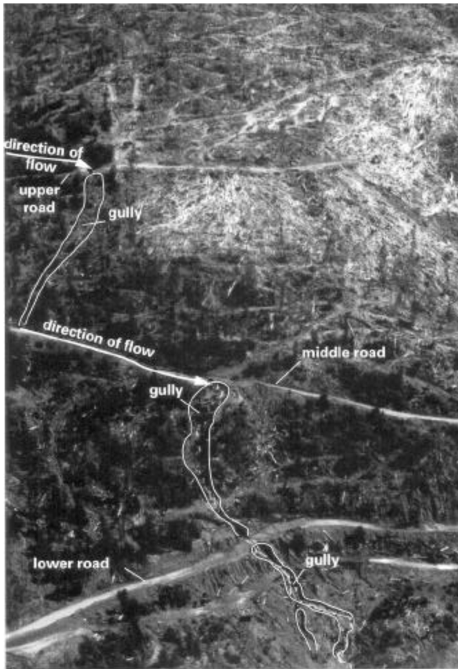
FIGURE 3.—Oblique aerial photograph of a roaded, clearcut hillslope in the lower Redwood Creek basin. Lack of culverts on the upper road resulted in large gully that extended from the end of switchback down to the middle road. The lack of a culvert at the stream crossing on the middle road caused diversion of flow down the ditch and across a road prism near center of the photograph, creating a large, visible gully extending down to and across the lower road system. Photograph was taken soon after the March 1972 storm.
